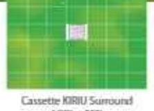
Cassette KIRIU Surround ADPI ~ 95%
